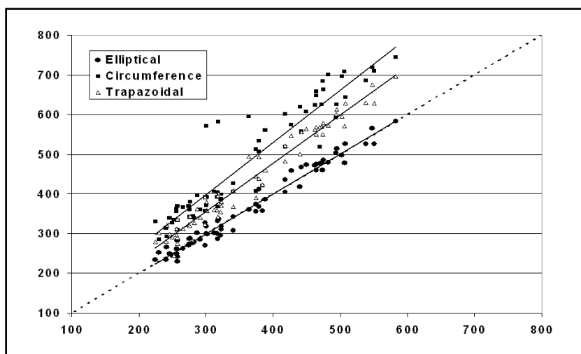
Fig. 5. Subject Hand Volumes. Relationship between paired-volumes as determined by water displacement (VW) and the elliptic (VE) trapezoidal (VT) and circumference (VC) algorithms. The solid lines are the linear regressions defined by the equations and parameters in the figure. The dashed line is a line of identity.
