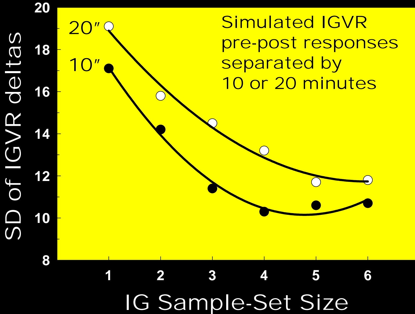
FIG 8 Paired-Difference SD
