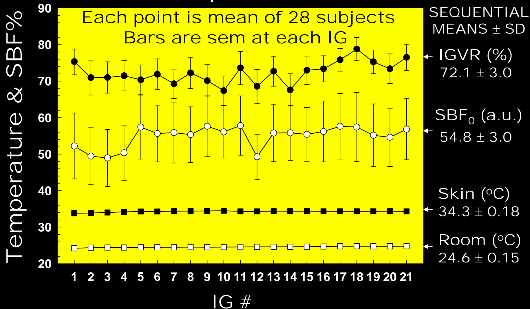
FIG 6 Sequential Values
